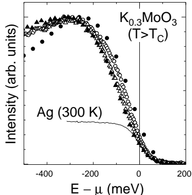
Figure 13: Angle integrated photoemission data of K_{0.3}MoO_3 in the normal metallic state. Filled circles: angle sum of data in Ref. [77] (also shown in Fig. 15), h\nu = 20 eV, \Delta E = 100 meV, \Delta\theta = \pm 10^\circ , T = 220 K. Empty circles: this work, h\nu = 13 eV, \Delta E = 27 meV, \Delta\theta = \pm 6^\circ , T = 250 K. Empty triangles and line: Ref. [13], h\nu = 21.2 eV, \Delta E = 33 meV, \Delta\theta = \pm 12^\circ , T = 300 K. Filled triangles: Ref. [75], h\nu = 21.2 eV, \Delta E = 20 meV, \Delta\theta = \pm 3^\circ , T = 313 K.
